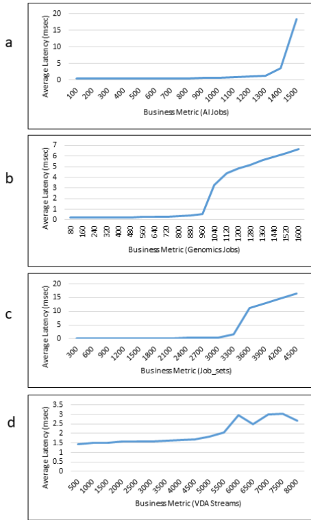
Figure 2: AI_Image, Genomics, EDA_Blended, and VDA SPEC Latency results
